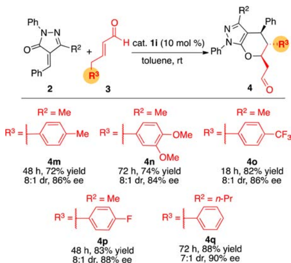
Scheme 3. Scope of Various Enal Reaction Partners a
