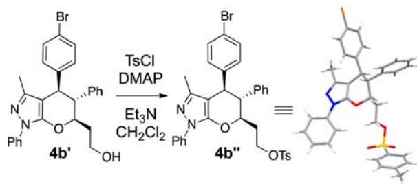
Scheme 4. Synthesis and X-ray Structure of 4b''
